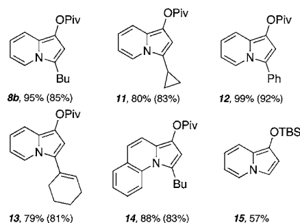
Figure 1. Pt(II)- and In(III)-catalyzed cycloisomerizations. Yields are indicated for reactions using \text{PtCl}_2 and \text{InCl}_3 (in parentheses). For a full description of reaction details, including the identity of propargylic ester substrates, see Supporting Information.
