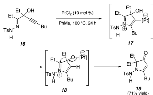
Scheme 3. Tandem Cyclization/1,2-Migration of 16
